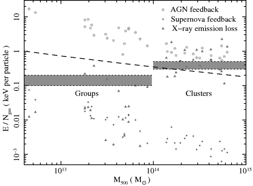
Fig. 2. Estimated energy feedback to the IGM by AGNs (circles) and supernova explosions (crosses), compared to the average gas energy excess of \approx 0.1 - 0.2 and \approx 0.3 - 0.5 keV per particle for galaxy groups and clusters (grey belts), respectively, the X-ray radiative loss since z = 2 (triangles), and the energy required to deviate scaling relations from self-similar predictions (dashed line; see Wang et al. 2010 for details).
