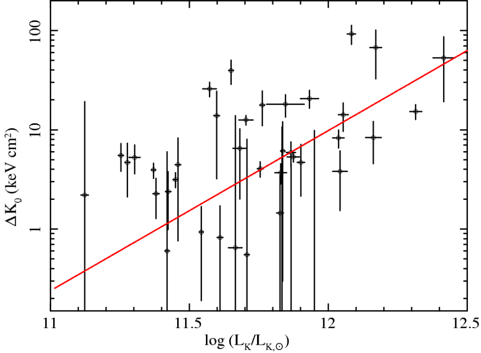
Fig. 1. Central gas entropy excess \Delta K_0 vs K -band luminosity L_K for the 40 CDGs of our sample (see Fig. 2 in Wang et al. 2010). The solid line shows the best-fit model \log(\Delta K_0) = -0.8 \pm 0.3 + (1.6 \pm 0.4)[\log(L_K/L_{K,\odot}) - 10.9] .
